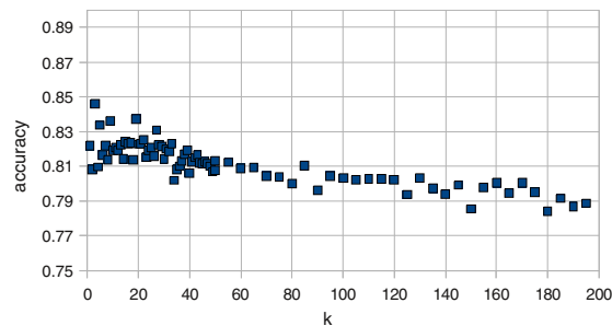
Fig. 8. The classification accuracy for the k -NN rule with the Music data
