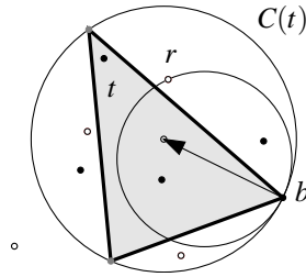
Figure 6: If Statement 1 of Lemma 3 is not true then P \neq Q .
